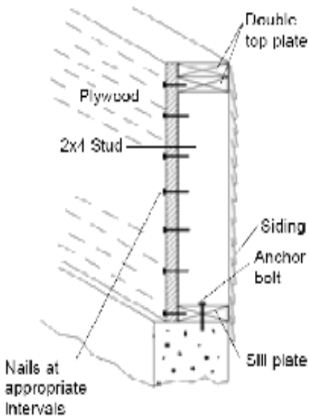
Figure 17—Plywood or diagonal sheathing strengthens weak cripple walls. If your home has a cripple wall between the foundation and the first floor, and the wall is not braced with plywood or diagonal sheathing, the house may fall or shift off its foundation during an earthquake.
